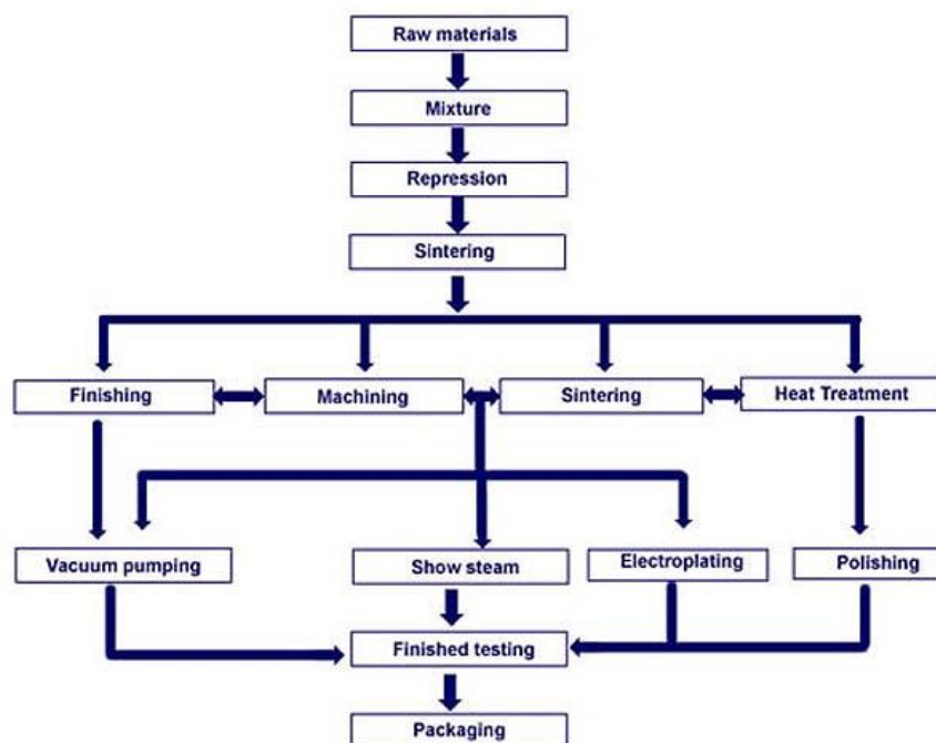
Fig. 1 Principle of powder metallurgy process [4, edited and supplemented by author]
